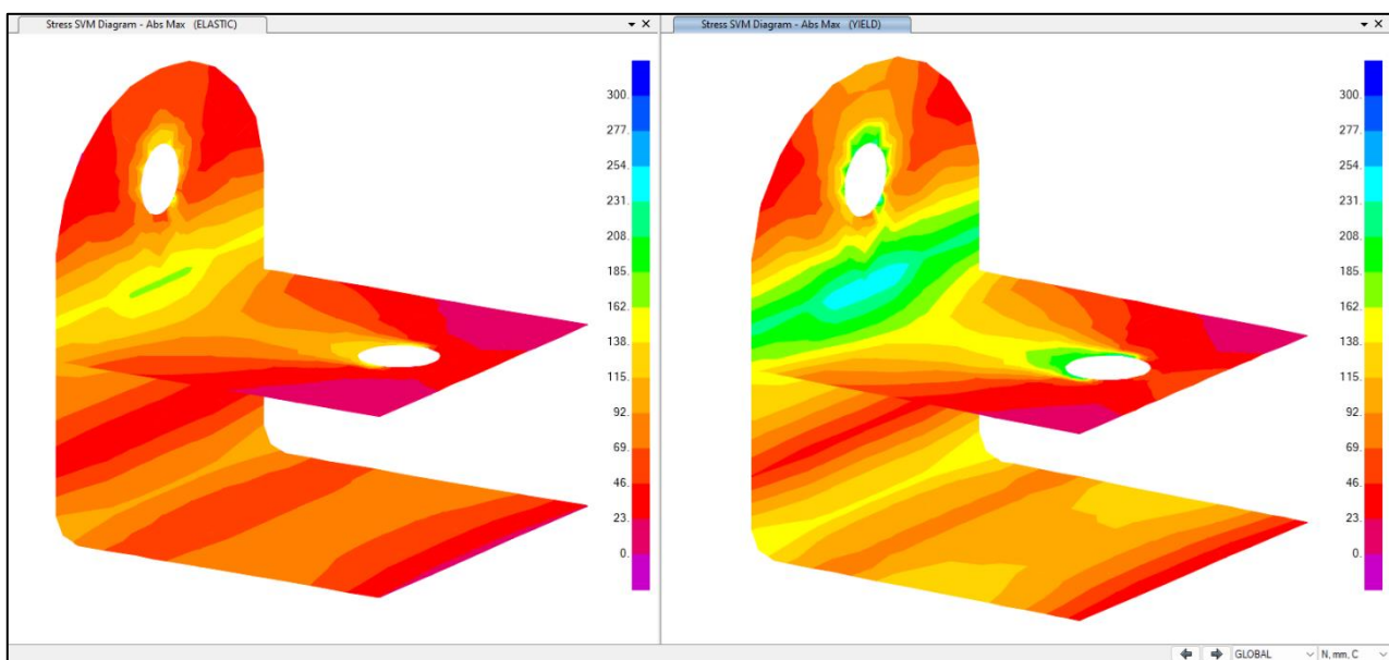
Figure 4.2: Von Misses stresses in Plate Clamp at Elastic and Yielded Condition per BS EN 13155:2020
