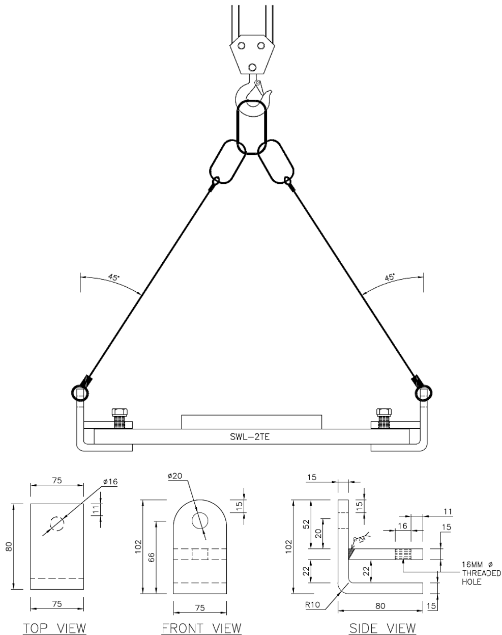
Figure 4.1: Details of Plate Clamp
